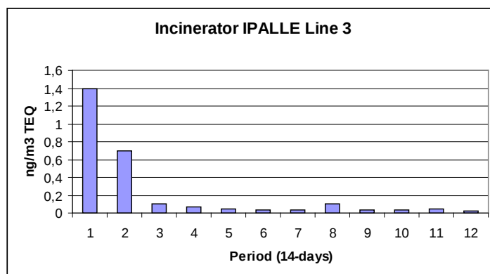
14 days emission values of incinerator 3 of IPALLE
