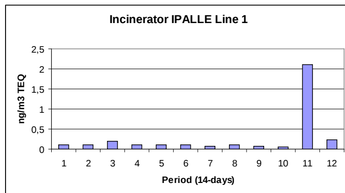
14-days emission values of incinerator 1 of IPALLE
