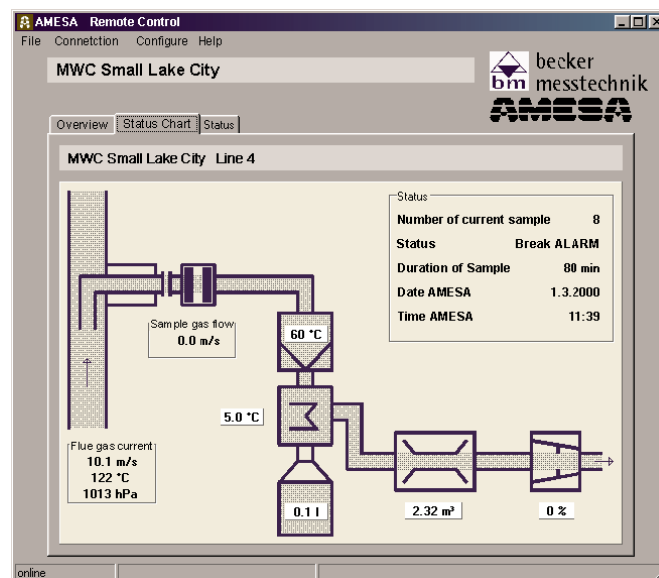
Status chart window of remote control software AMLEIT
