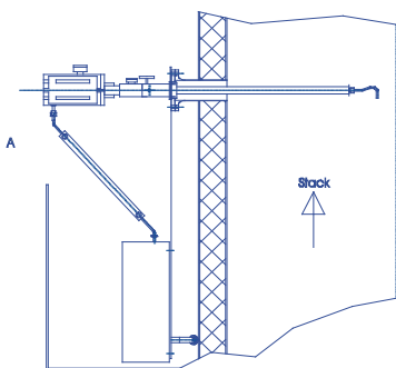
Installation drawing of the high-dust-probe
